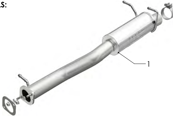
1. MUFFLER ASSEMBLY
